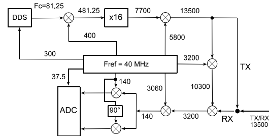
Figure 2: ASIRAS frequency plan (all frequencies are in MHz). (From RST (2007))
