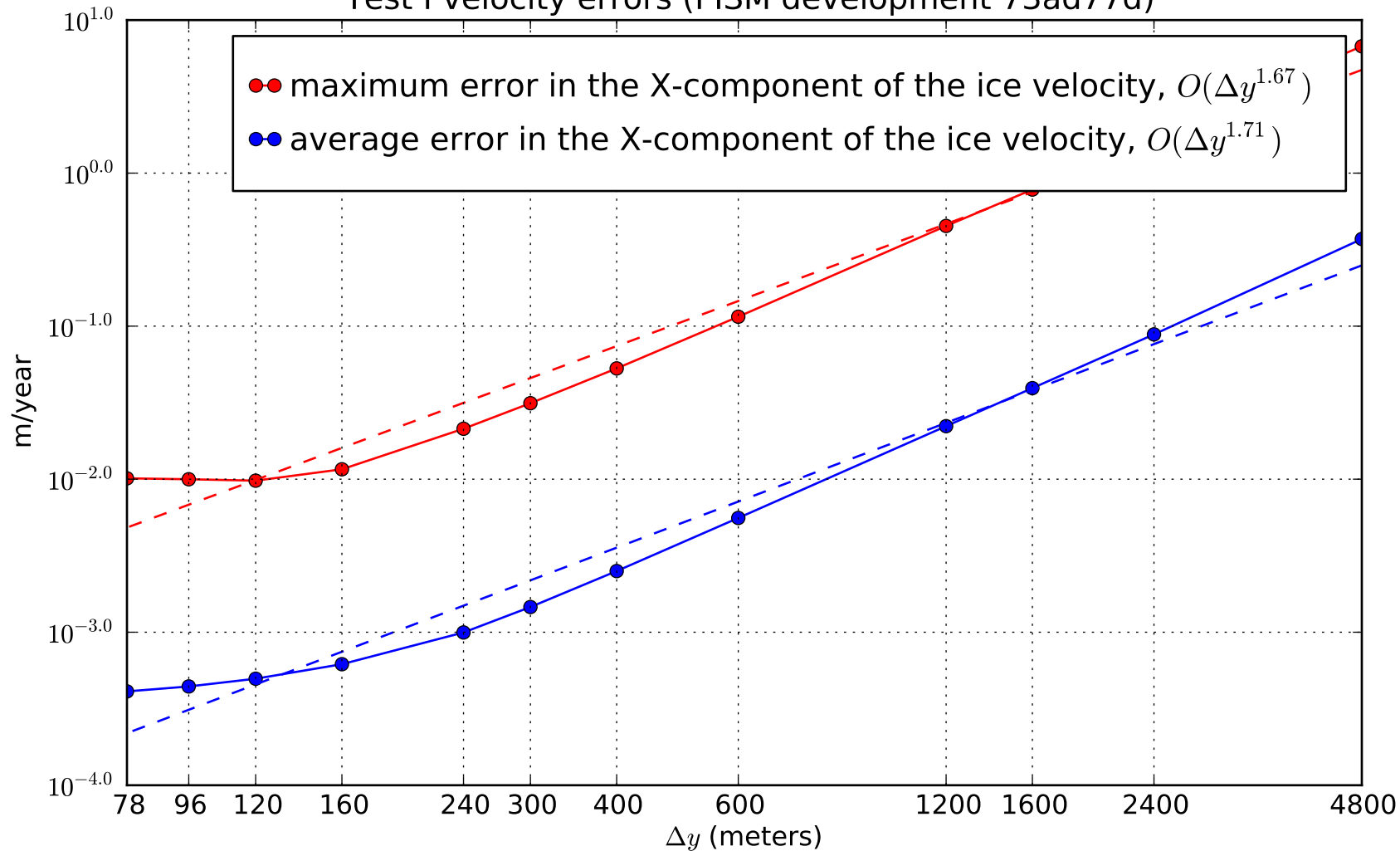
Test I velocity errors (PISM development 73ad77d)
