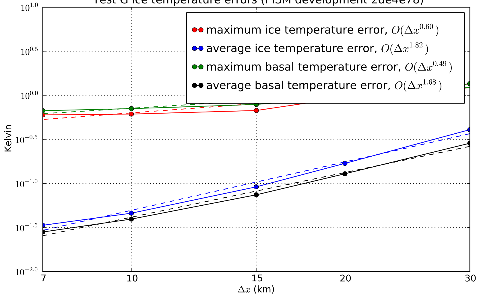
Test G ice temperature errors (PISM development 2de4e78)
