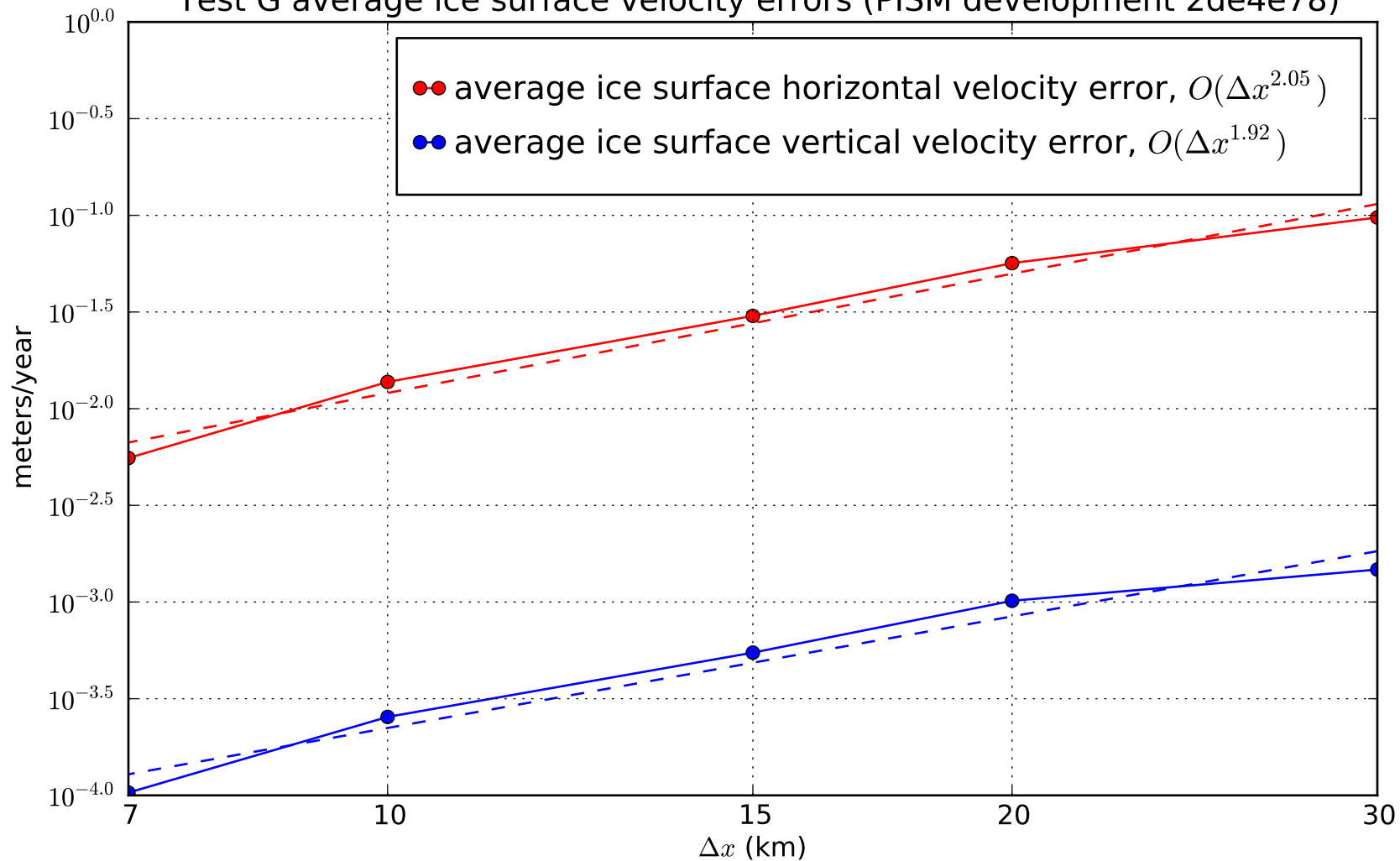
Test G average ice surface velocity errors (PISM development 2de4e78)
