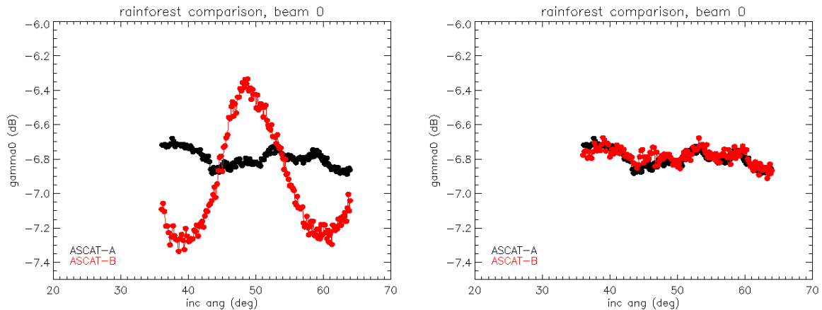
Figure 2: Comparison of ASCAT-A and B data over the Amazon rainforest before (left) and after (right) cross calibration.
