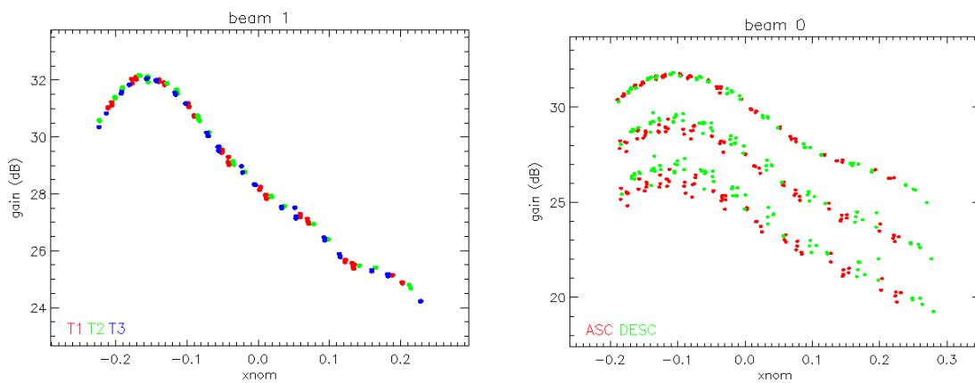
Figure 4: (left) transponder data LEFT MID beam, showing minor distortion and (right) transponder data in LEFT FORE beam at three different azimuth angles, showing differences between ascending and descending passes.
