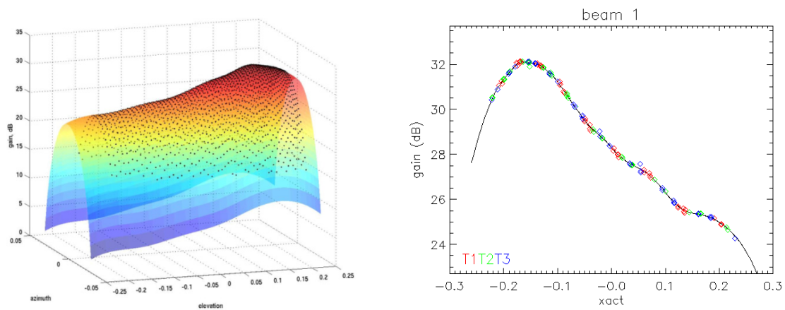
Figure 5: (left) Example gain pattern as a function of antenna elevation and azimuth angles and (right) a section through LEFT MID beam gain pattern as a function of elevation angle.
