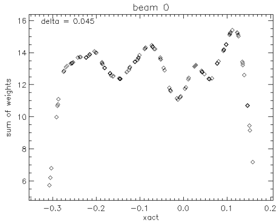
Figure 7: Sum of the weights used to fit the low order polynomial in the kernel smoothing for the LEFT FORE beam.
