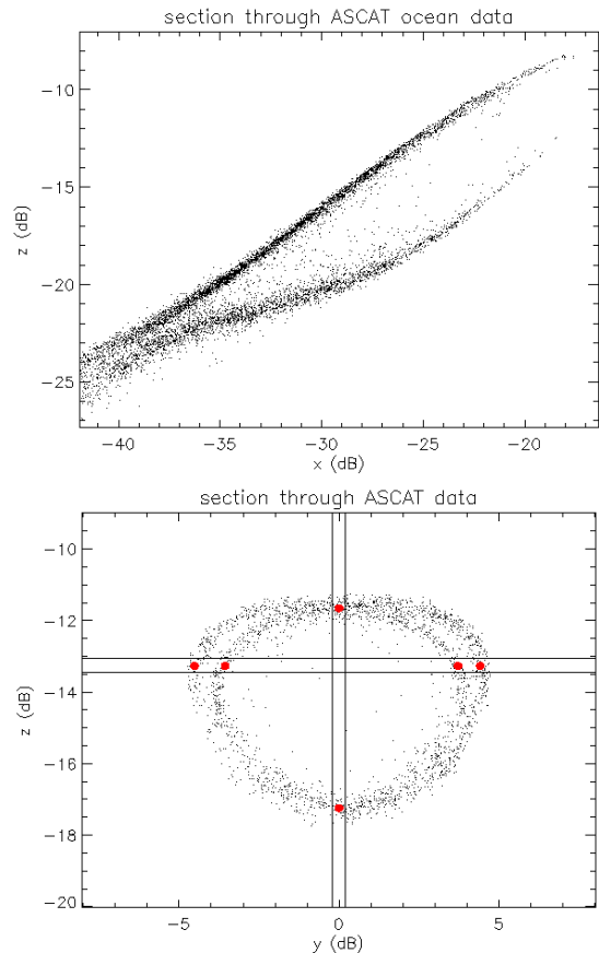
Figure 9: Example of sections through a month of ASCAT-B data from the open ocean with the position of maximum data density in two slices marked in red. These sections vary with incident angle.
