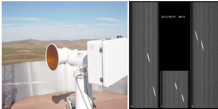
Figure 3: (left) Transponder on site in Turkey and (right) transponder signals in ASCAT calibration data.
