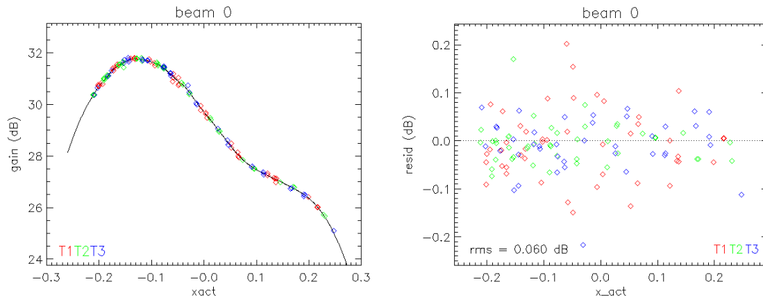
Figure 6: (left) Transponder data with the fitted gain model and (right) the residual between data and model, for the LEFT FORE beam
