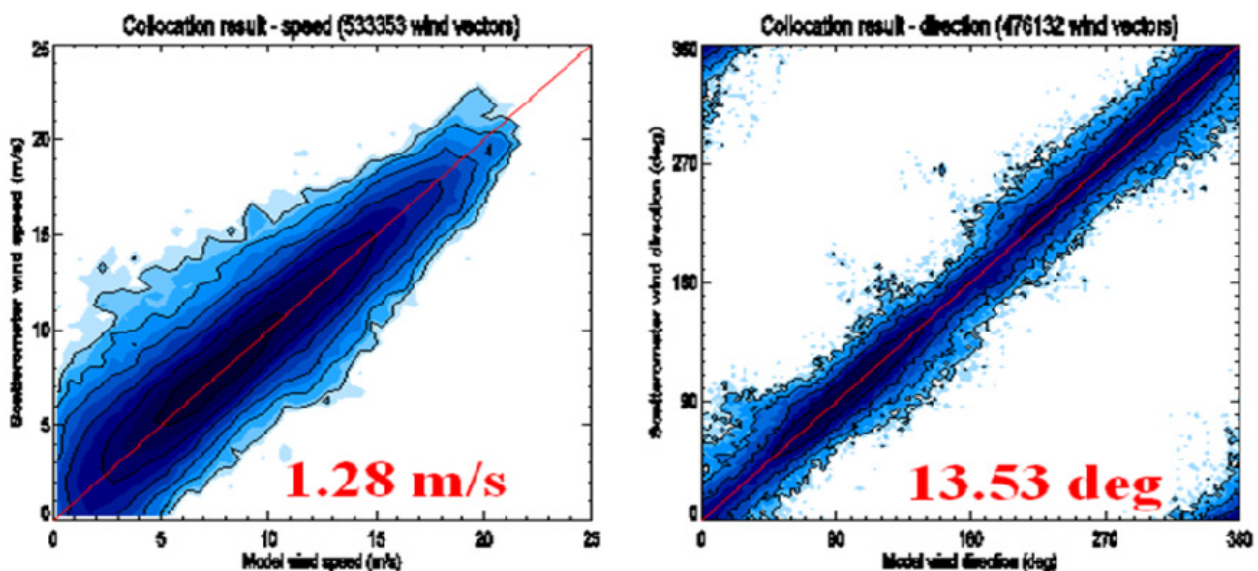
Figure 11: Difference in wind speed and direction between wind vectors derived from ASCAT-B data and ECMWF NWP output. Plots courtesy of Royal Netherlands Meteorological Institute.
