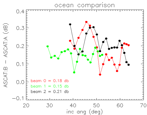
Figure 10: Difference in the cone position for open ocean NRCS from ASCAT-A and B during February 2013.
