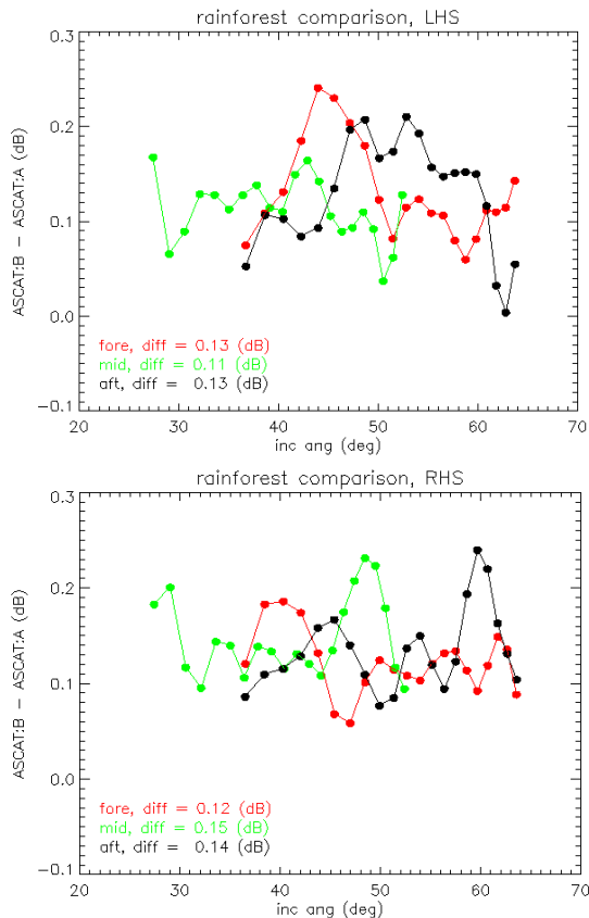
Figure 8: Difference in mean \gamma_0 between the rainforest data from ASCAT-A and B during February 2013.
