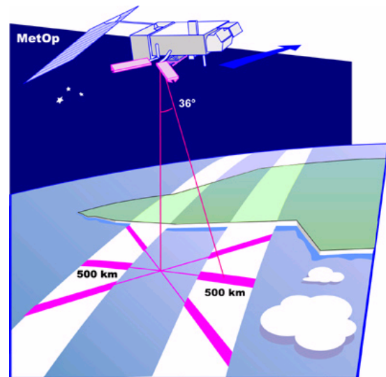
Figure 1: Schematic showing the viewing geometry of the ASCAT (picture provided by ESA).
