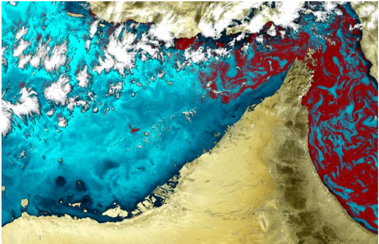
Figure 3. Large Red Tide in the Oman sea and Persian Gulf. Composite image resulting from the processing of a MERIS data acquired 22/11/2008. The land is obtained using the Tristimulus algorithm (L1 data). The sea image is obtained using the following band combination: Red=Red tide Index, Green=band ratio 490/555nm, Blue=band ratio 510/555nm. The image can be interpreted as follow: Red colour - HABs (Red Tide), Brown colour - non-HABs, Dark blue colour - high suspended sediments and dissolved materials, Cyan colour - relatively clear waters. Clouds are in white color
