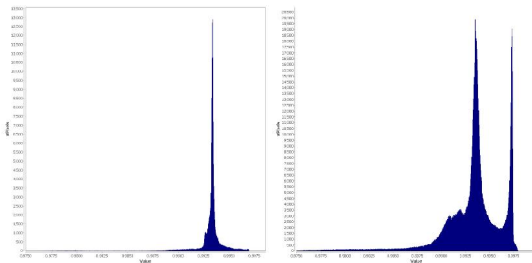
Figure 4. Histograms of the Red tide Index (RI) for two MERIS images dated 13/05/2009 with no alga bloom (left) and 22/11/2012 when a large Red Tide interested both Oman sea and Persian Gulf (right). Both histograms show a peak around 0.994, while the right one shows a second peak after 0.997 common to other scenes with a Red Tide occurring.
