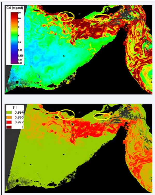
Figure 5. Chlorophyll map (top) ad HAB detection map (bottom) from a MERIS scene acquired the 30/12/2012. The HAB map was obtained applying three threshold values to the RI: red=high probability, green=no HAB. The yellow circles evidence different behaviours of the two parameters.
