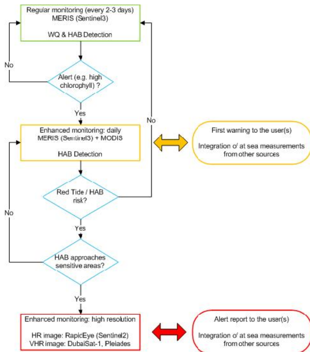
Figure 2. Flowchart describing the UAE Service Trial concept for HAB/Red Tide monitoring and alert
