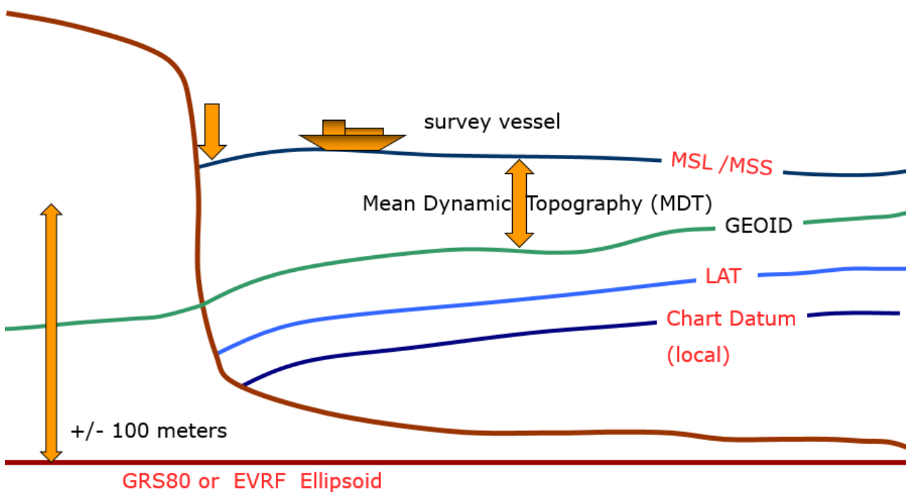
Figure 1.0: Sketch of the DTU18 MSS relative to the GRS80 ellipsoid
