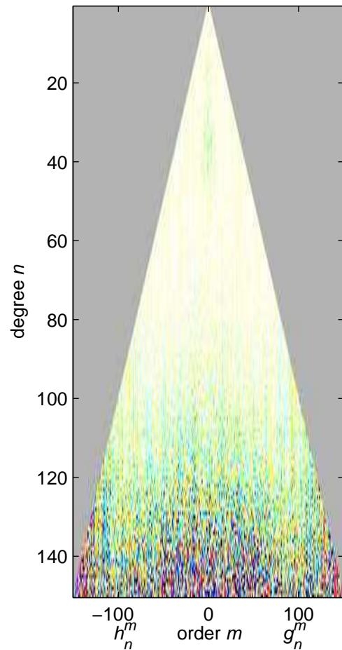
Final Model, N = 41, M = 0
