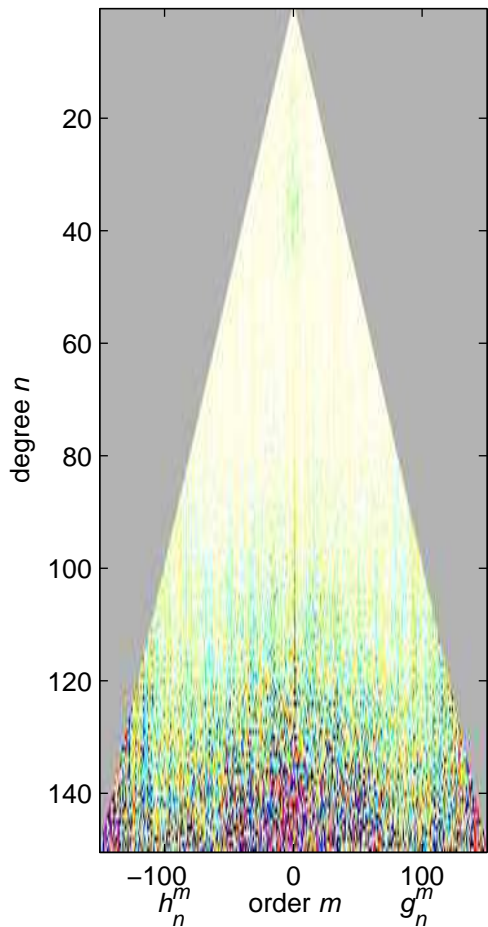
Final Model, M = 11
