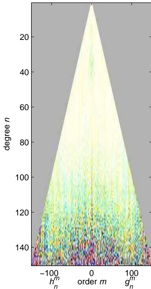
Final Model, M = 41-5
