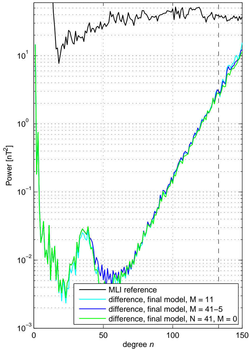
MLI Power Spectrum
