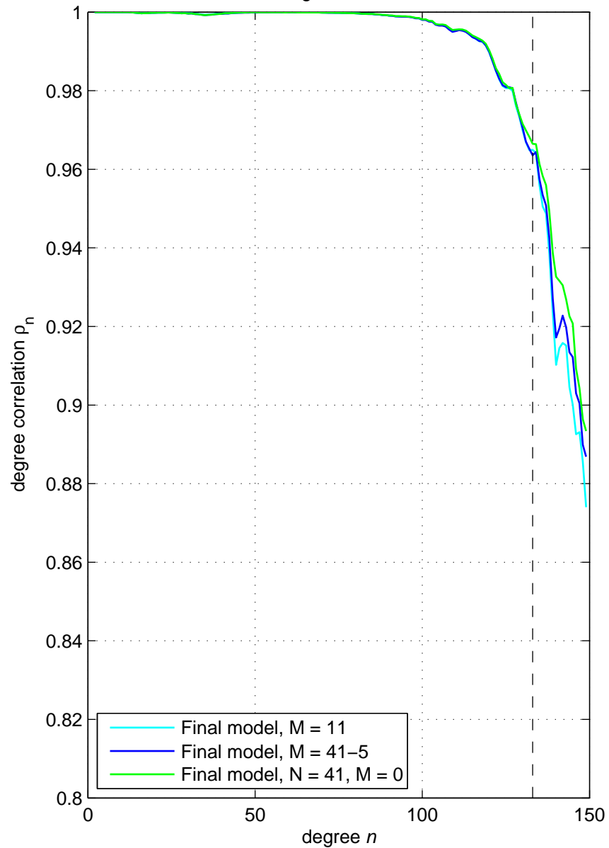
MLI Degree Correlation
