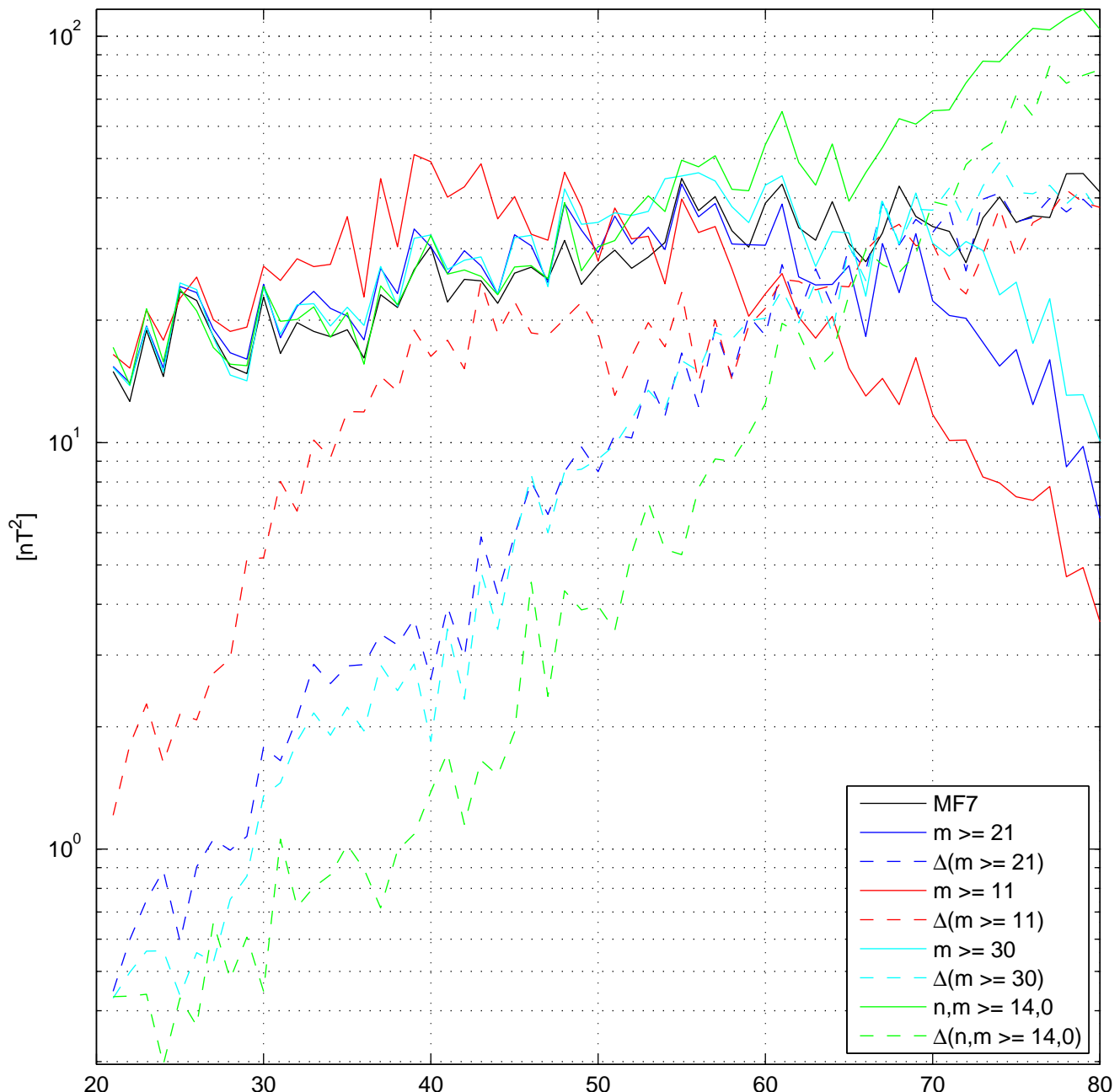
MLI Powerspectra
