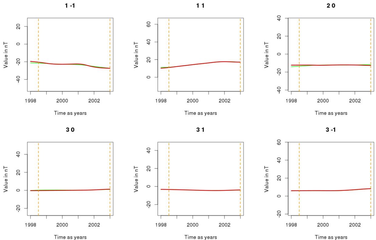
Figure 4-8: Time series of secular variation Gauss coefficients, the green line is the behaviour of the reference model over the full time span, the red line is the data period covered used for model estimation, the vertical dashed lines indicate the data period covered.
