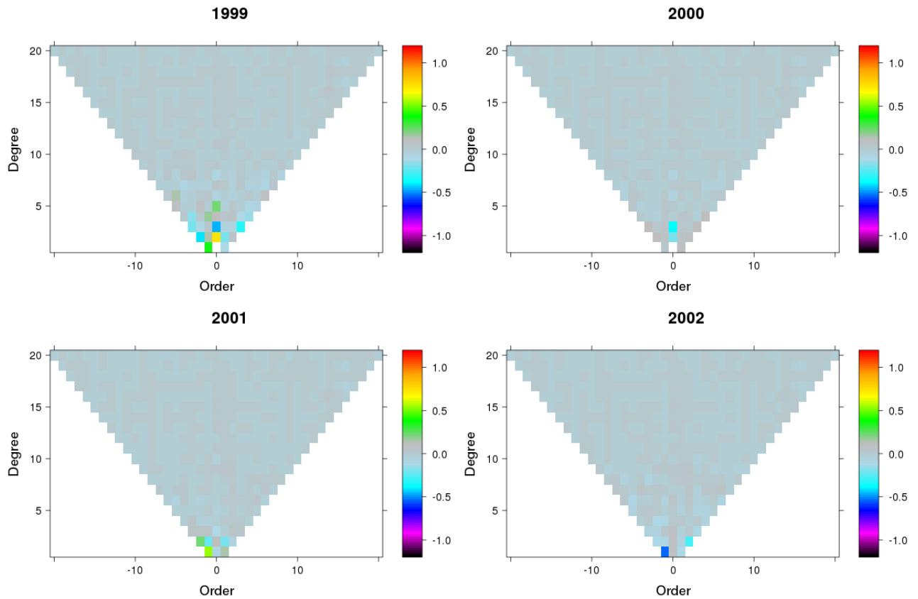
Figure 4-6: Visualisation of secular variation differences between inverted model and reference field in a triangular order over degree scheme in nT/yr.
