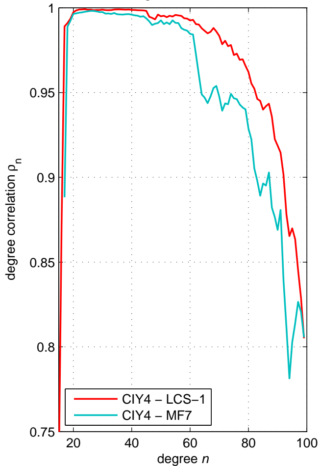
Degree Correlation
