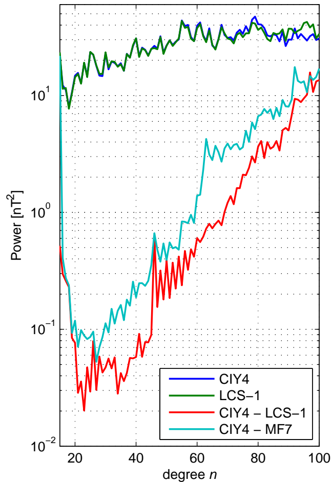
Power Spectra
