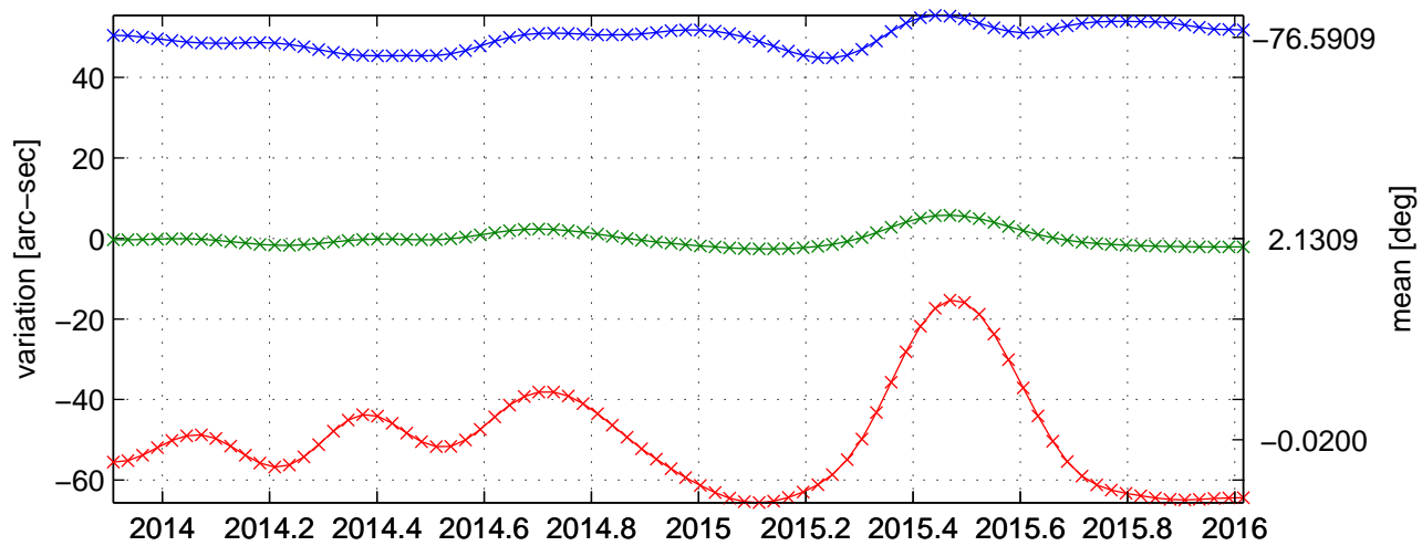
Swarm B, 2-3-1 Euler Angle Variations
