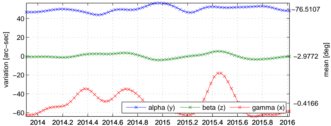
Swarm A, 2-3-1 Euler Angle Variations
