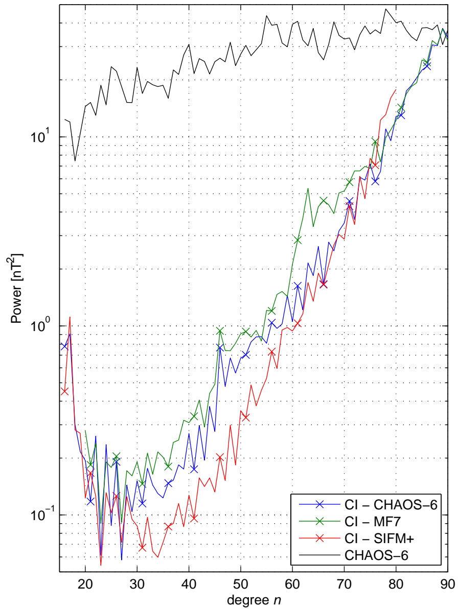
MLI Power Spectra
