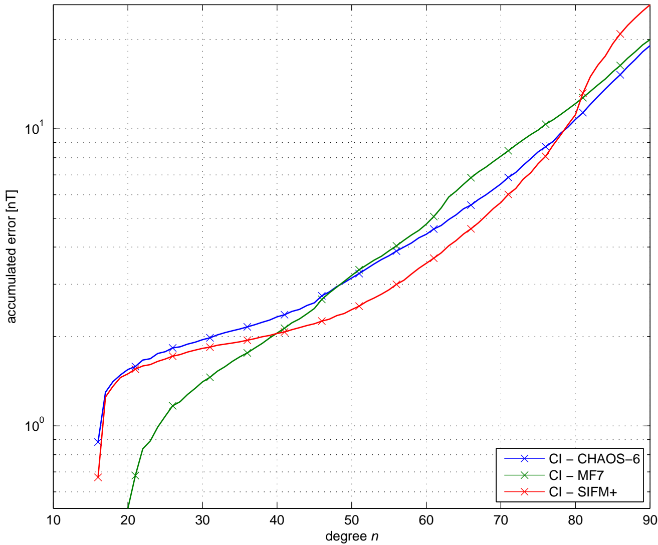
MLI Accumulated Error on Ground
