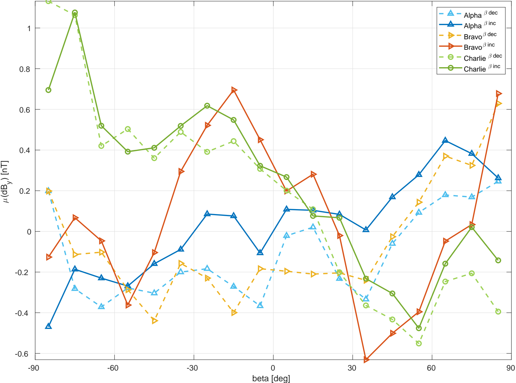
Swarm, CIY8 Residuals, beta-bin Averages
