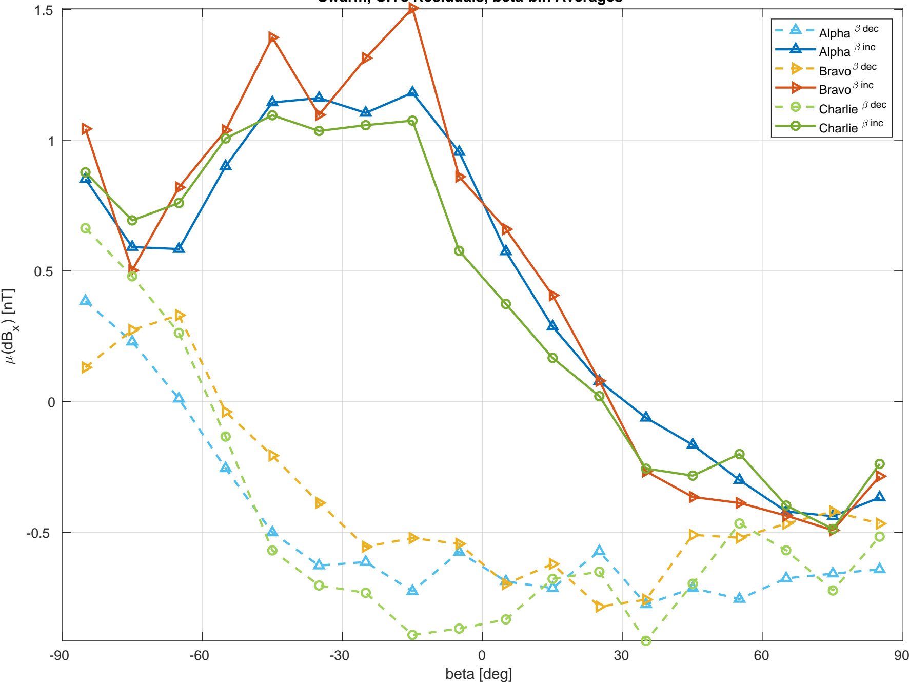
Swarm, CIY8 Residuals, beta-bin Averages
