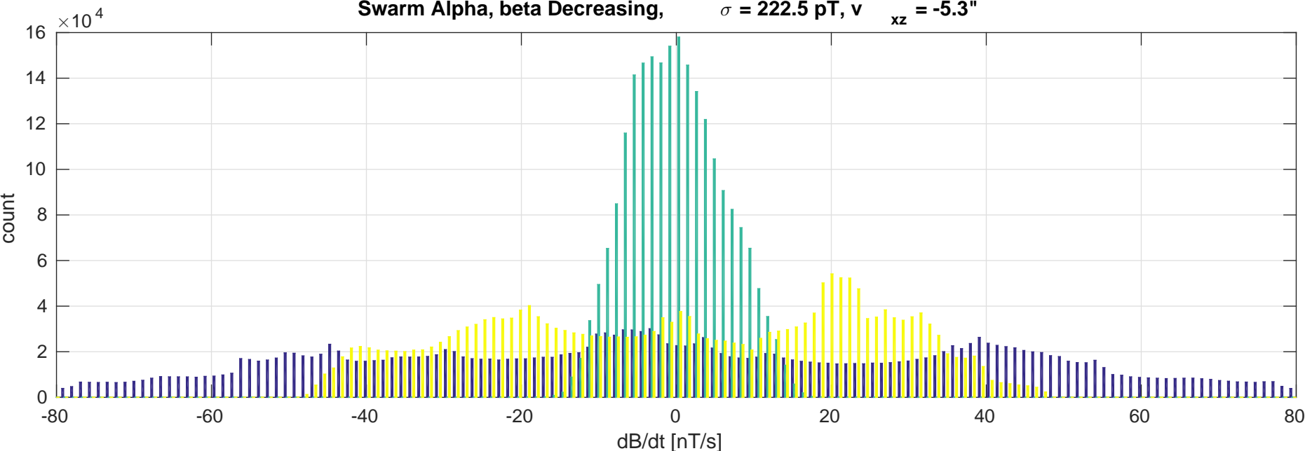
Swarm Alpha, beta Decreasing, \sigma = 222.5 pT, v_{xz} = -5.3''
