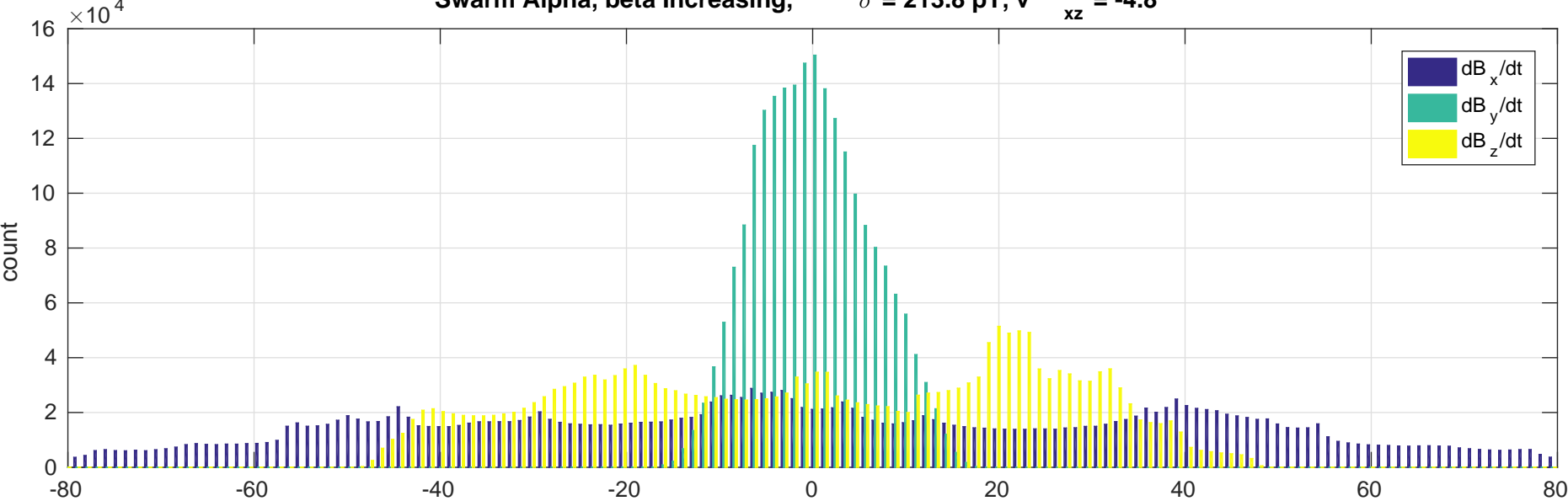
Swarm Alpha, beta Increasing, \sigma = 213.8 pT, v_{xz} = -4.8''
